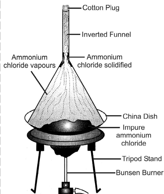
Sublimation of ammonium chloride
